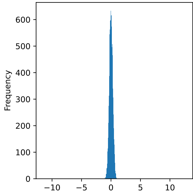
\sigma=0.3 Variance: 0.0908
