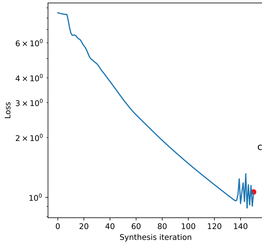
Representation error
