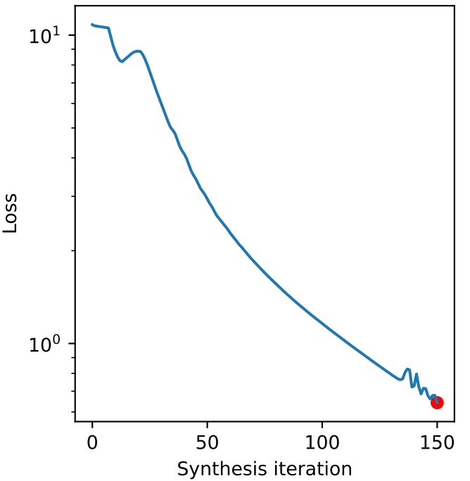
Representation error
