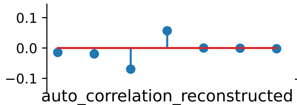
pixels+var_highpass
