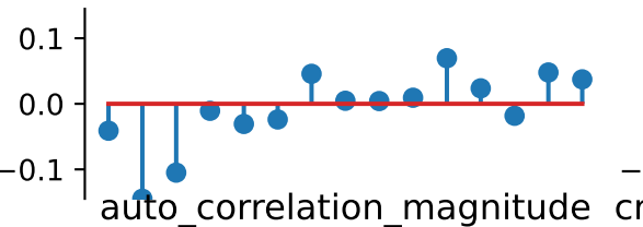
std+skew+kurtosis recon
