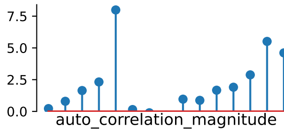
std+skew+kurtosis recon
