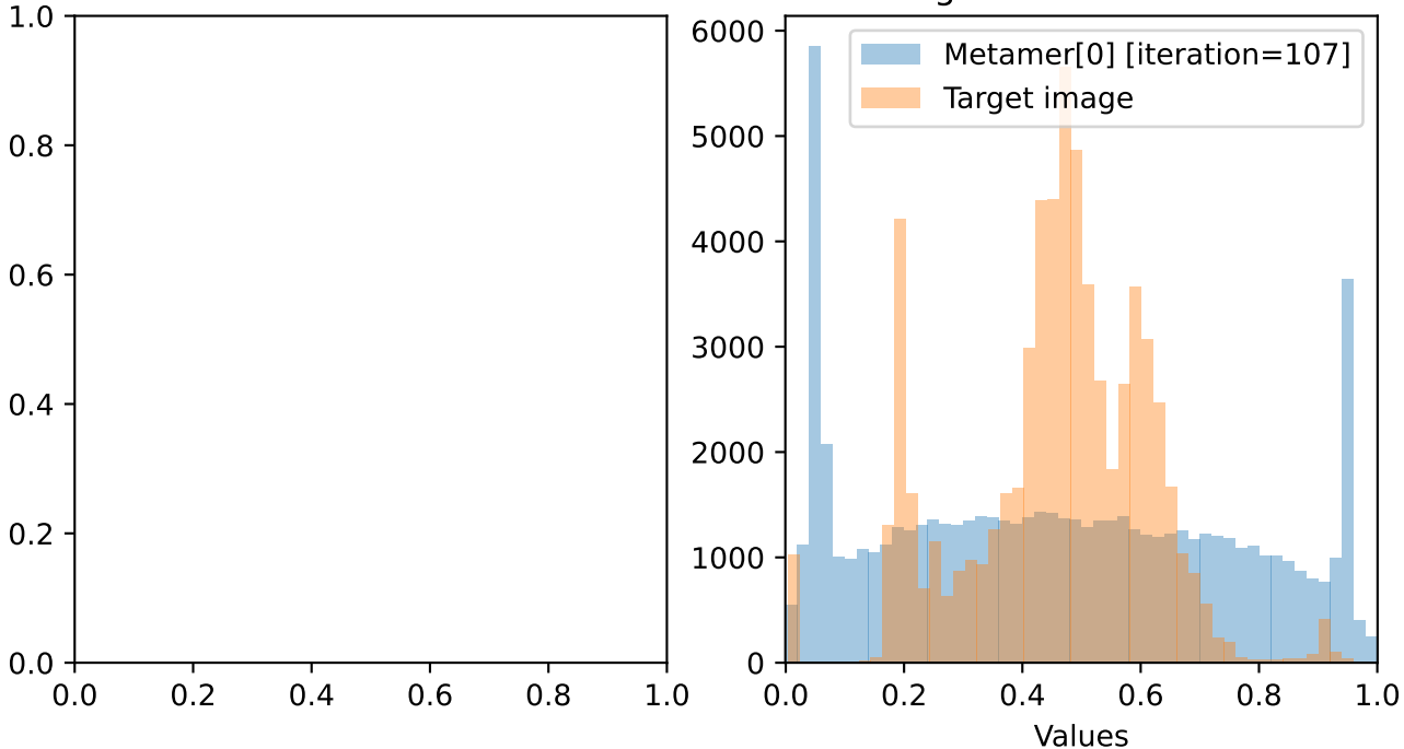
Histogram of tensor values
