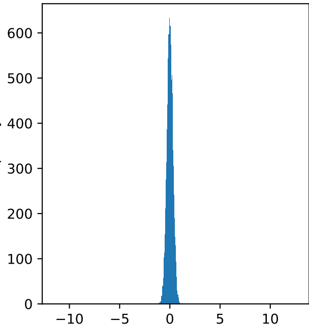
\sigma=0.3 Variance: 0.0908
