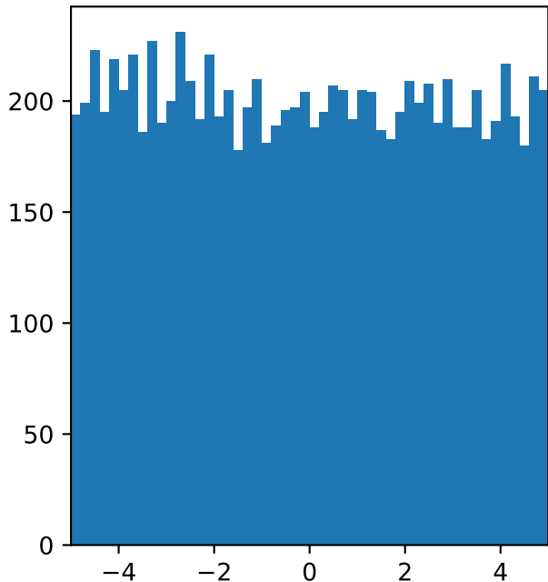
Platykurtic (Uniform) Kurtosis: 1.7859
