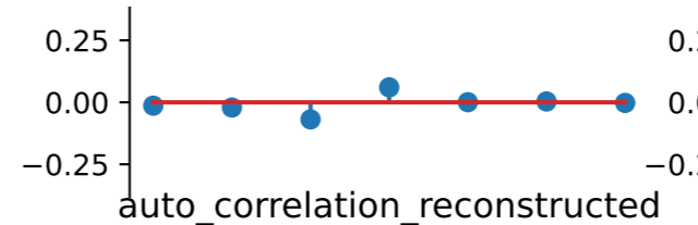
pixels+var_highpass
