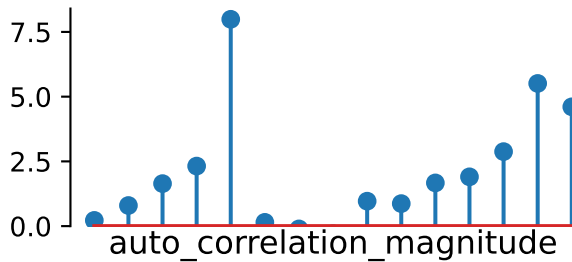
std+skew+kurtosis recon
