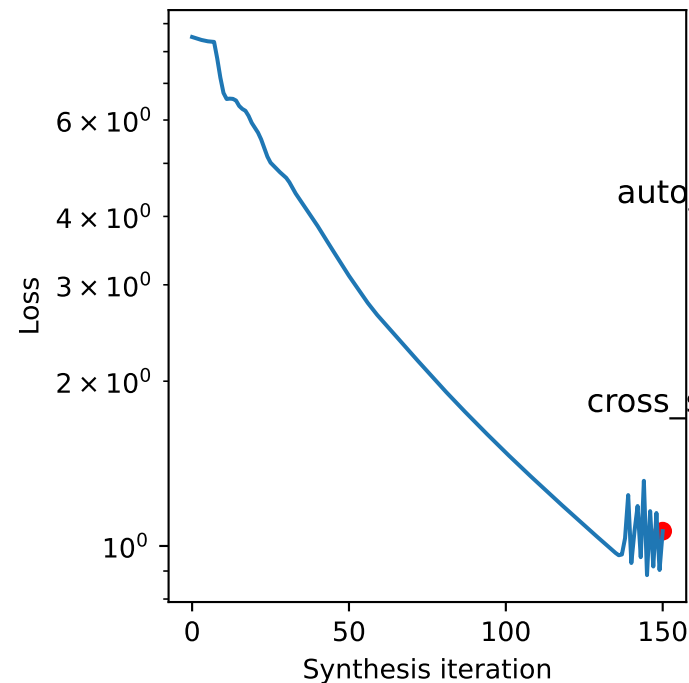
Representation error
